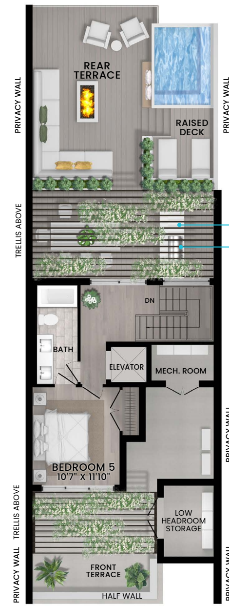
4TH FLOOR ROOFTOP PLAN BEACH FRONT MIDDLE UNIT
