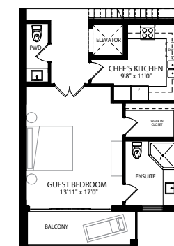
PARTIAL 2ND FLOOR PLAN BEACH FRONT MIDDLE UNIT OPTIONAL CHEF'S KITCHEN
