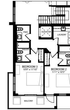
PARTIAL 2ND FLOOR PLAN BEACH FRONT EXT/INT END UNIT OPTIONAL 2 BEDROOMS
