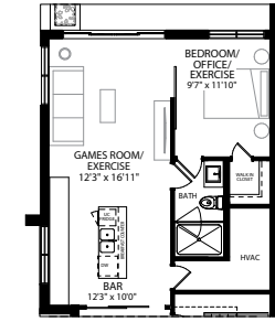
PARTIAL 1ST FLOOR PLAN BEACH FRONT EXT END UNIT OPTIONAL GAME ROOM/BEDROOM
