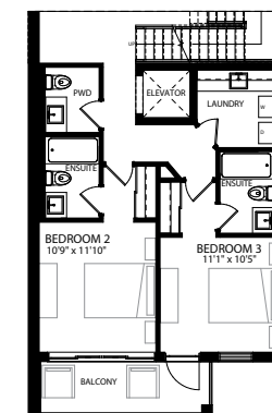
PARTIAL 2ND FLOOR PLAN BEACH FRONT MIDDLE UNIT OPTIONAL 2 BEDROOMS
