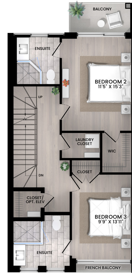
2ND FLOOR PLAN POOL FRONT MIDDLE UNIT
