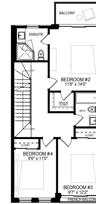
OPTIONAL 2ND FLOOR PLAN POOL FRONT MIDDLE UNIT OPTIONAL 4 BEDROOM HOME ELEVATOR NOT POSSIBLE FOR TOWNHOUSE WITH THIS OPTIONAL FLOOR PLAN
