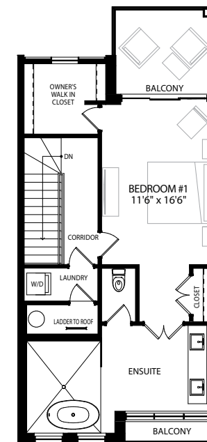
3RD FLOOR OPTIONAL STANDARD LOCK-OUT 3 BEDROOM PLAN (NO ROOFTOP)
